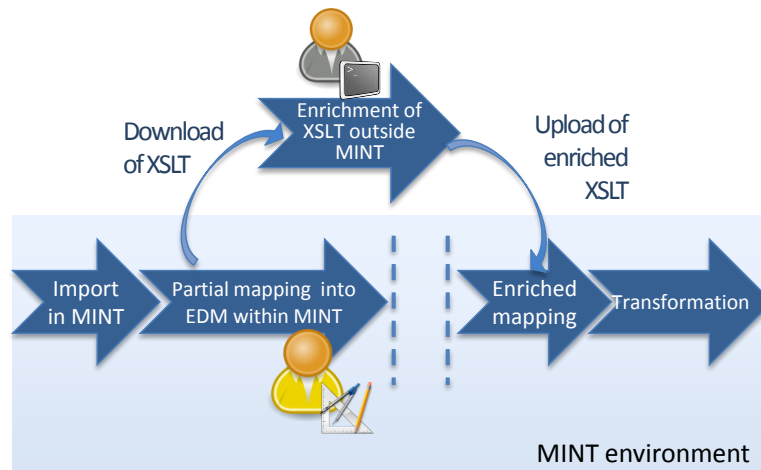
Figure 5. Mapping enrichment
