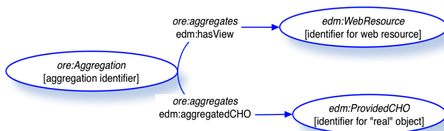
Figure 3. Core EDM classes
