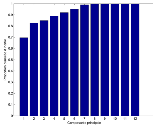
(c) Inerties des axes factoriels
